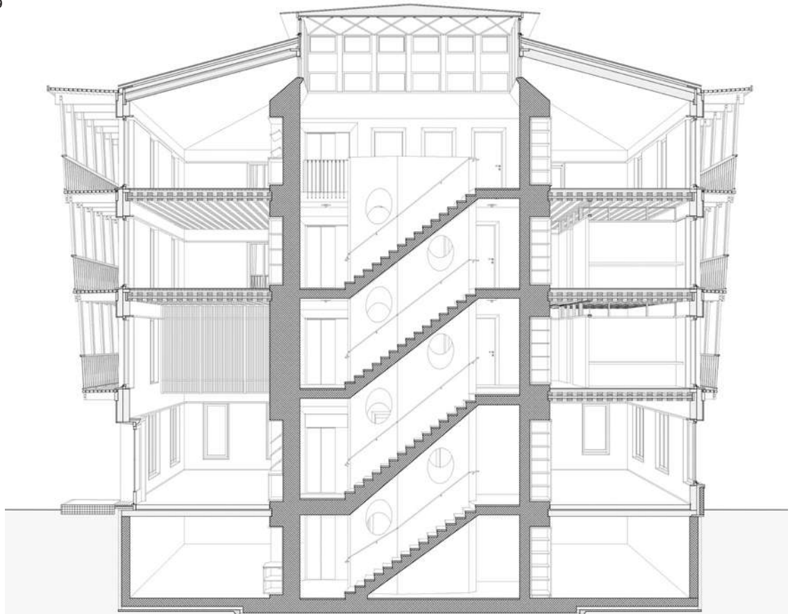
Fig. 6 Detail of the façade.
